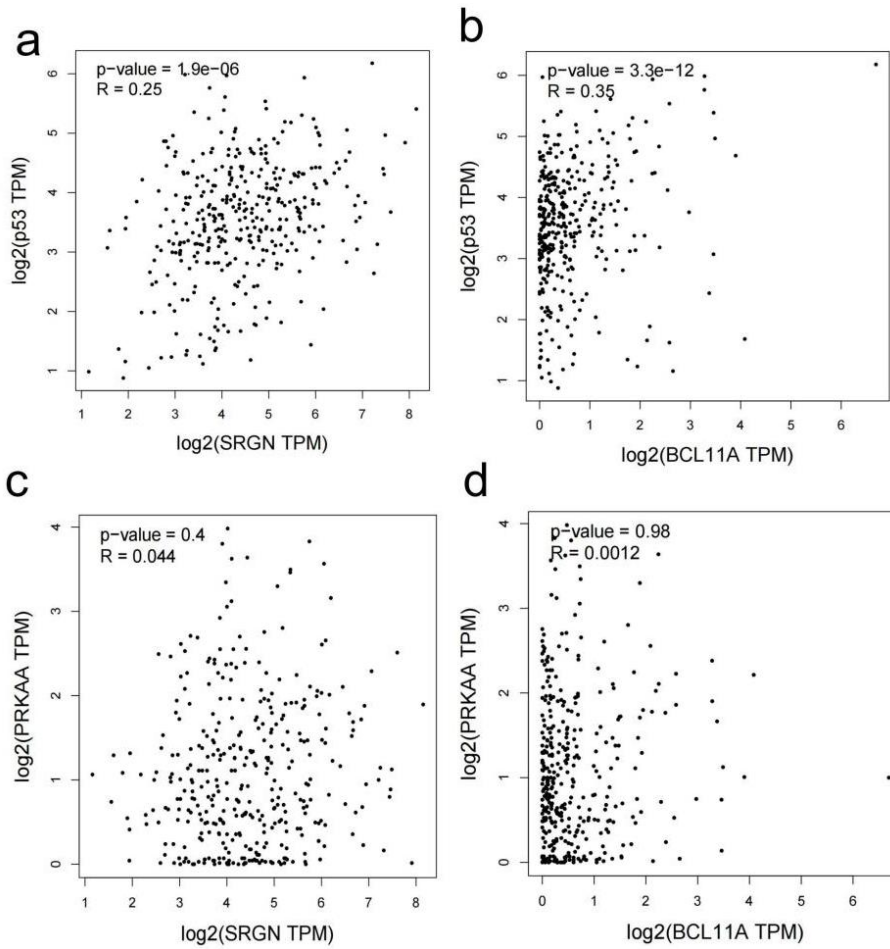
Figure S1. Correlation analysis shows a significant association of p53 with (a) SRGN and (b) BCL11A, but not for AMPK \alpha (PRKAA) with (c) SRGN or (d) BCL11A in HCC.
