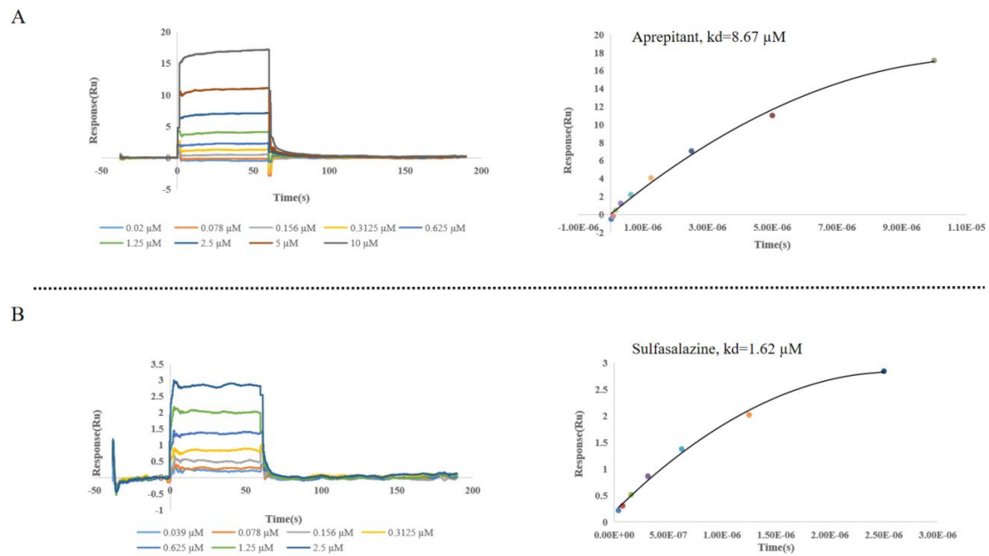
Figure 2. SPR results for Aprepitant and Sulfasalazine.
