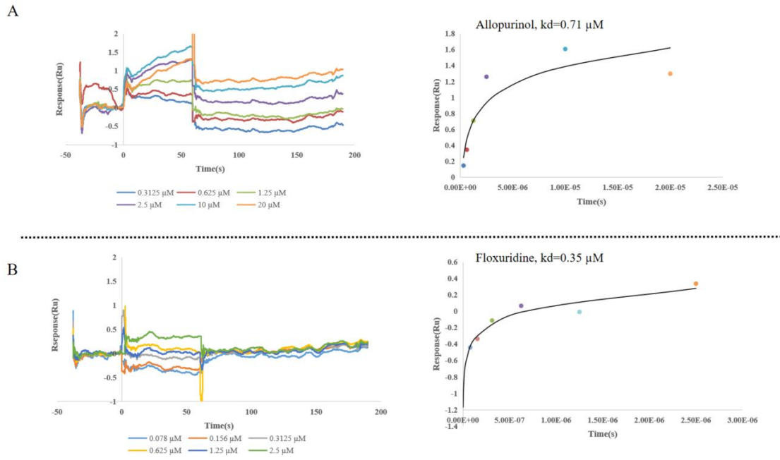
Figure 1. SPR results for Allopurinol and Floxuridine.
